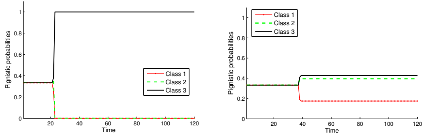
Figure 18: Credal classification results of two crossing targets: target 1 (on the left) and target 2 (on the right).
