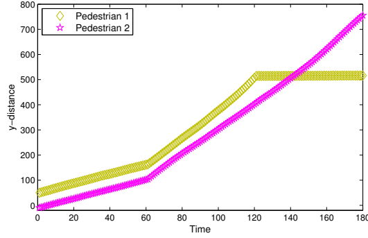
Figure 19: Pedestrians trajectories.
