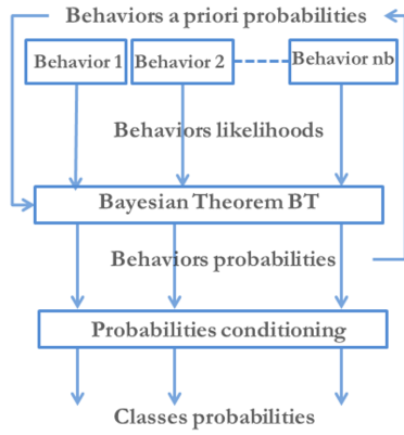
Figure 7: Bayesian classification.
