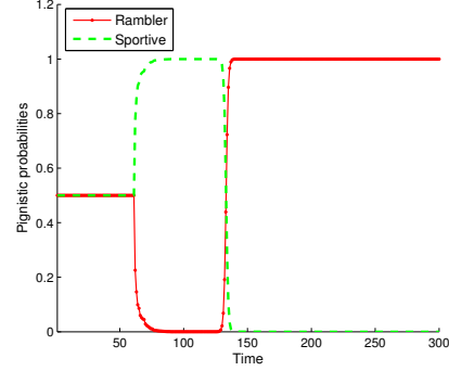
Figure 23: Instantaneous belief ( m_k ) discounting, with \lambda = 0.9 .
