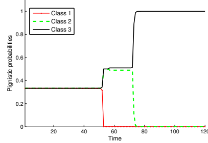
Figure 15: Target 2 credal classification.
