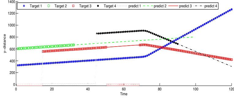
Figure 4: y-direction evolutions over time of 4 targets.
