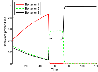
Figure 13: Behaviors probabilities of target 2.
