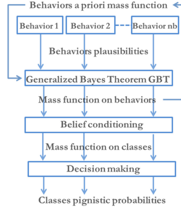
Figure 8: Credal classification.
