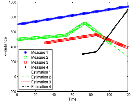
Figure 11: Targets measurements and estimations on x positions over time.
