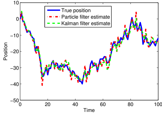
Figure 1: Kalman filter vs Particle filter.
