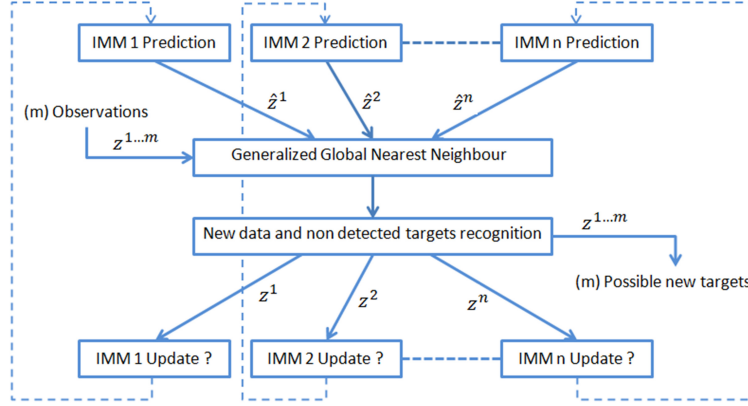
Figure 6: Multi-target tracking algorithm architecture.
