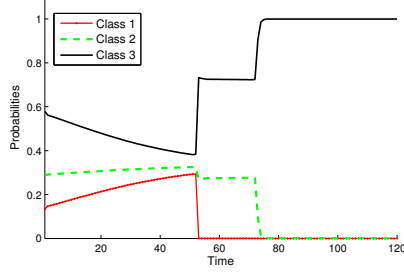
Figure 14: Target 2 Bayesian classification (after conditioning).
