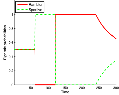
Figure 22: Cumulative belief ( m_{k-1} ) discounting, with \lambda = 0.9 .
