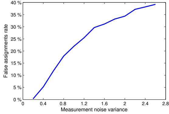
Figure 16: Rate of false assignments of GNN algorithm for two closely moving targets, with different sensor noise values.
