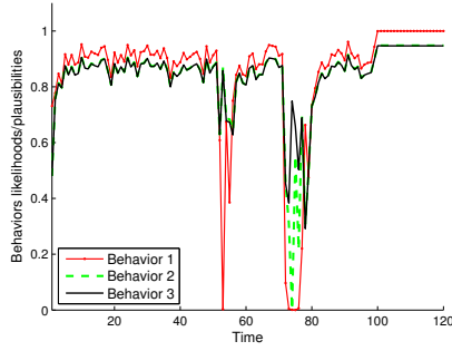
Figure 12: Behaviors likelihoods/plausibilities of target 2.
