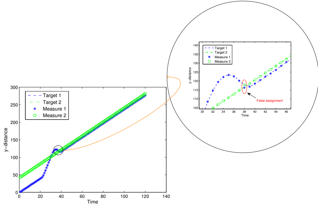
Figure 17: False assignment of the measurements of a fighter and an unknown aircraft.
