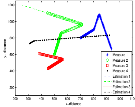
Figure 10: Targets measurements and estimations on x and y positions.
