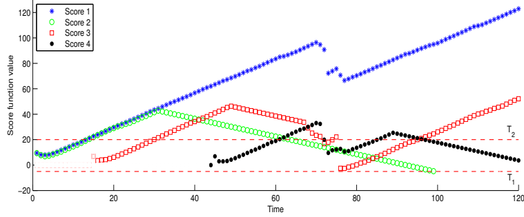
Figure 5: Targets score functions.
